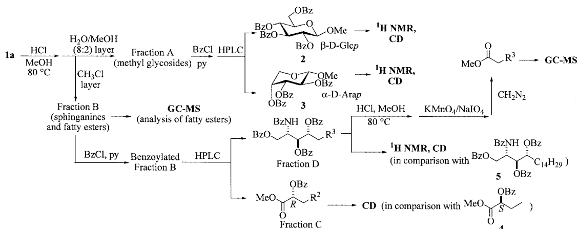
Scheme 2. The new microscale degradation procedure for glycolipids
